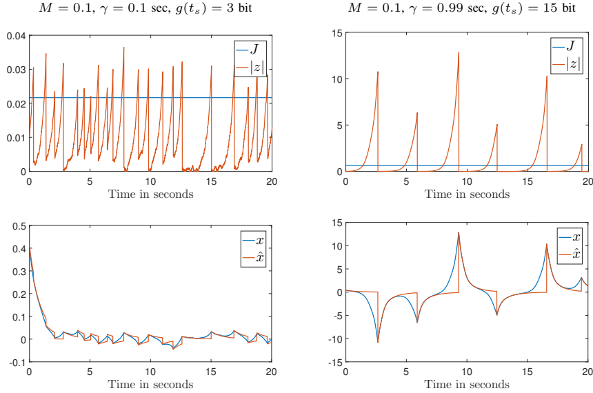
Fig. 7. Simulation results for stabilization of the plant (40). We used the following parameters for the simulation: sampling time \delta = 0.005 , simulation time T = 20 , u(t) = -4\hat{x}(t) , \alpha = 0.01 , packet size (39), and triggering threshold J = (e^{3\gamma} - 1)M/3 + 0.01 .
