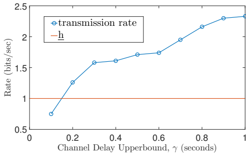
Fig. 8. Information transmission rate in simulations compared to the \underline{h} (41). We used the following parameters for the simulation: sampling time \delta = 0.01 seconds, simulation time T = 100 seconds, u(t) = -2\hat{x}(t) , z(0) = 0.01 , M = 0.05 , \alpha = 0.01 , packet size (39), and triggering threshold J = (e^{3\gamma} - 1)M/3 + 0.05 . Note that the rate calculated from simulations can not start at \gamma = 0 because the minimum channel delay upper bound is equal to two sampling time.
